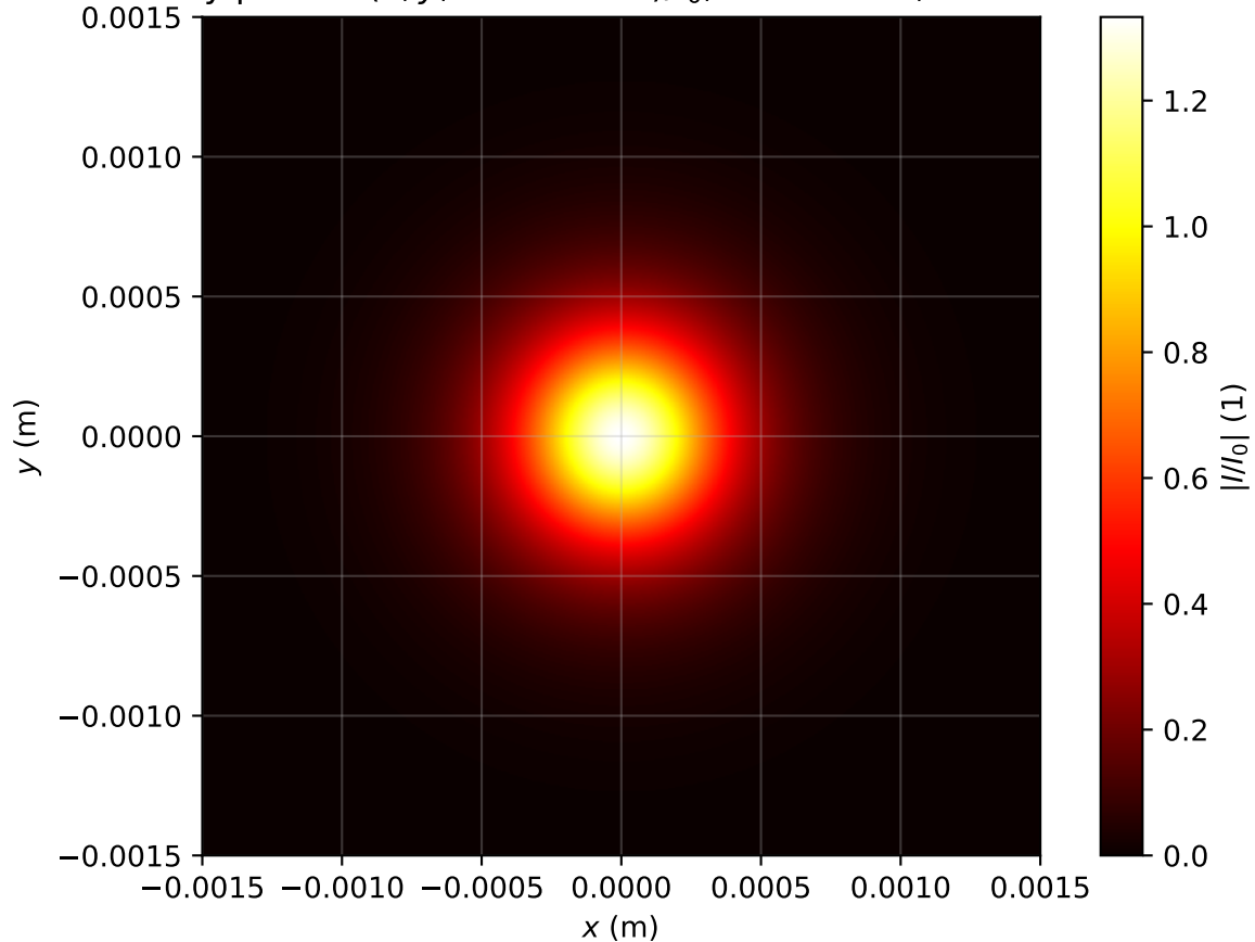
Intensity profile I(x, y, z = 1.194m)/I_0 , Pin=0.8Pcr, artificial time
